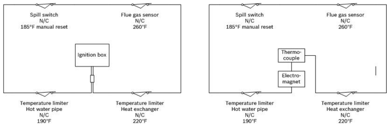
425HN and 1600H wiring Fig. 13 Safety circuit wiring diagram
