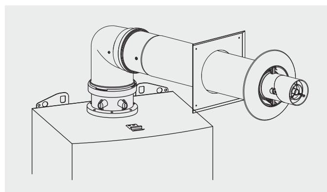
Fig. 10 completed adapter and concentric assembly
