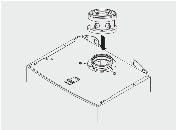
Fig. 4 Installing adapter
