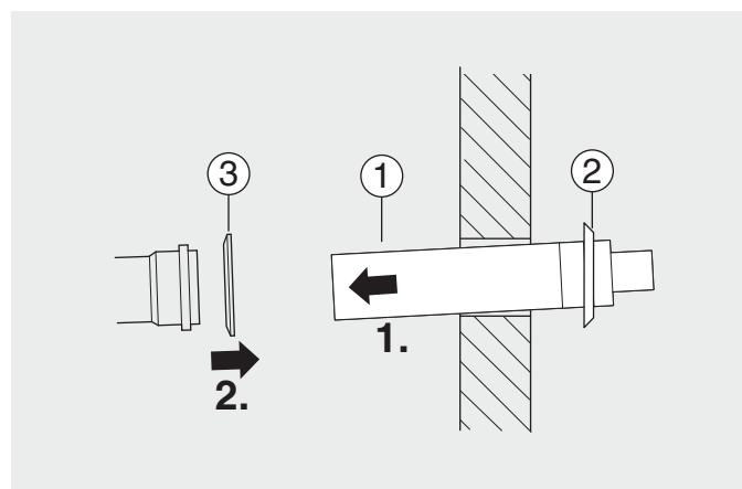
Fig. 9 Inserting termination from the outside
