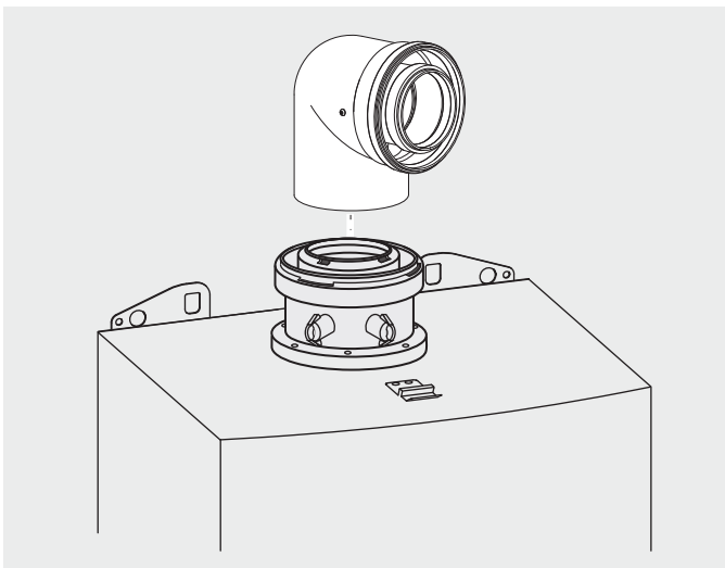
Fig. 5 Installing elbow
